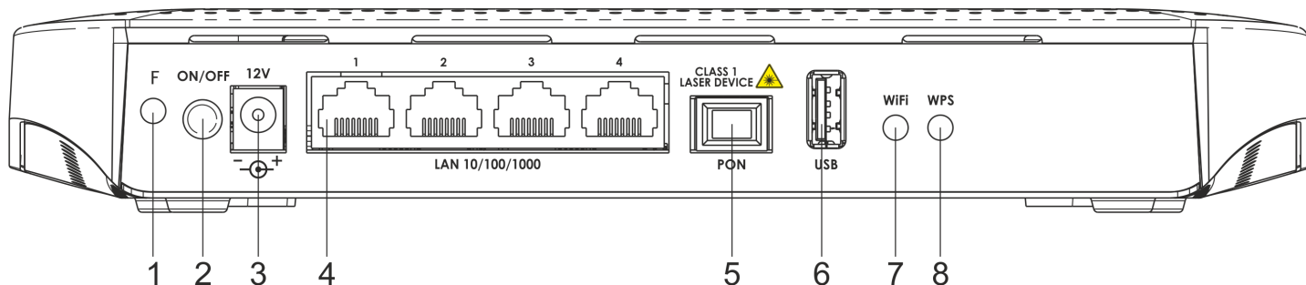
Figure 7 – NTU-RG-5440G-Wac, NTU-RG-5440G-WZ, NTU-RG5420G-Wac, NTU-RG5420G-WZ, NTU-RG5440G-Wac rev.B, NTU-RG5440G-WZ rev.B rear panel layout
